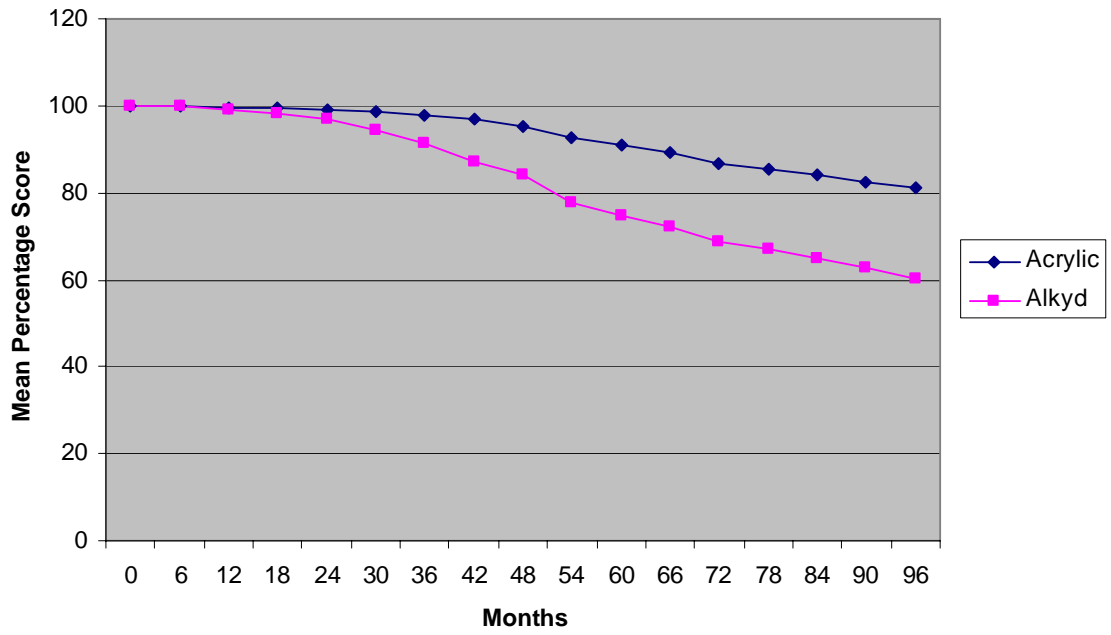
Paint Flaking vs. Paint Type
