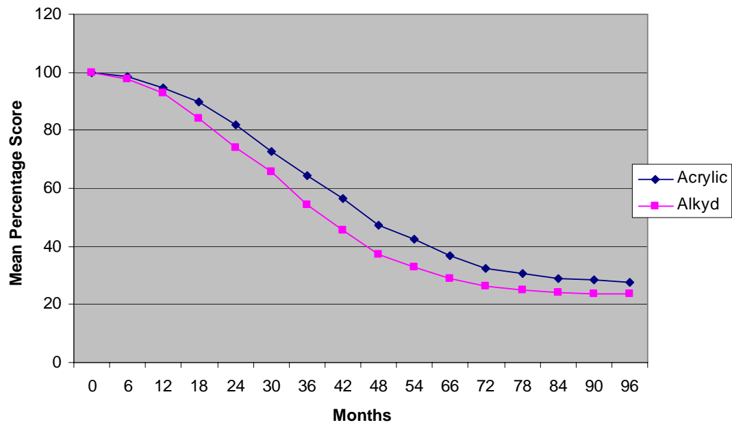
Paint Cracking vs. Paint Type
